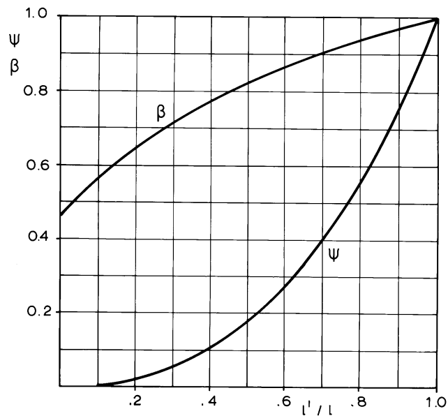
Figure 7 Determination of spring stiffness
