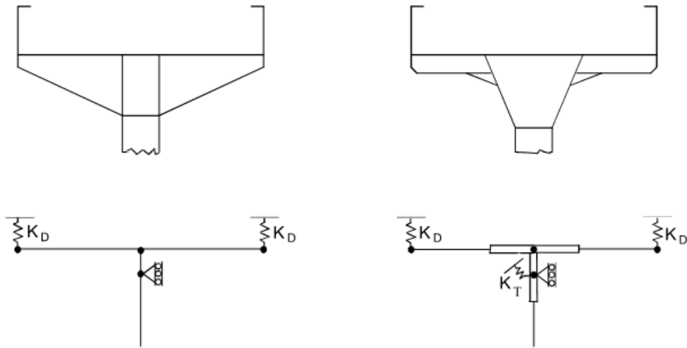
Figure 18 Spring support by hatch end coamings
