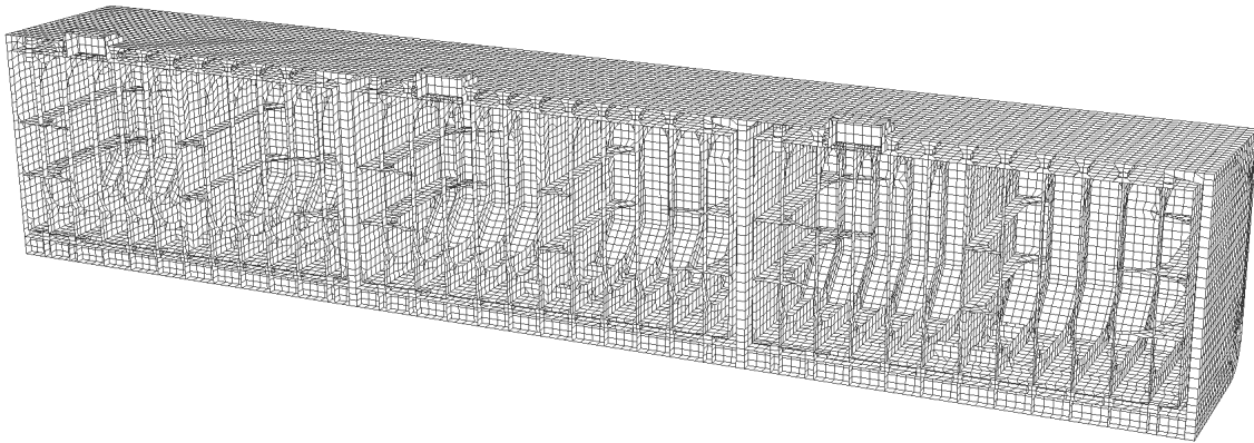
Figure 3 Example of 3 cargo hold model within midship region of a LPG carrier (independent tank design) (shows only port side of the full breadth model)
