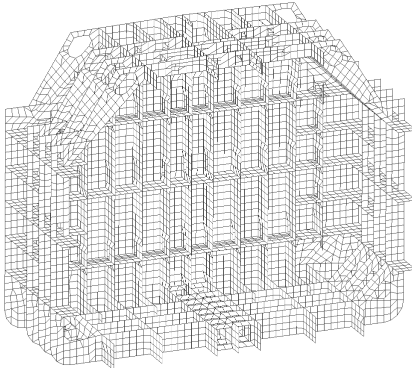
Figure 13 Example of FE mesh arrangement of cargo hold structure for a gas carrier ship
