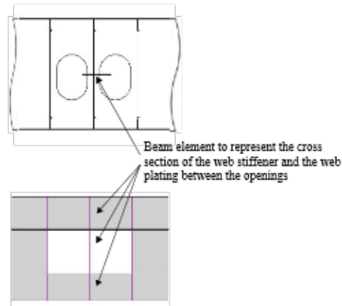
Figure 16 Modelling in way of sequential openings
