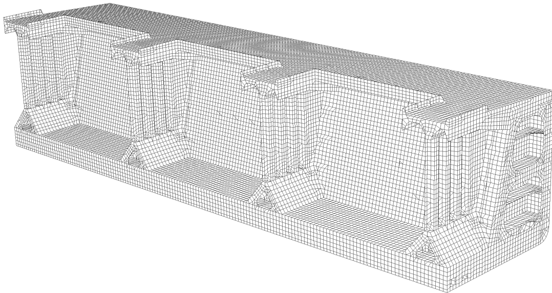
Figure 2 Example of 3 cargo hold model within midship region of an ore carrier (shows only port side of the full breadth model)
