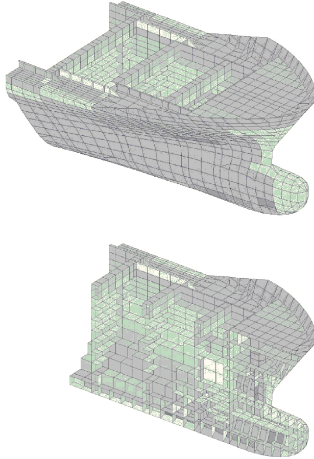
Figure 7 Typical foreship mesh used for global finite element analysis of a container ship
