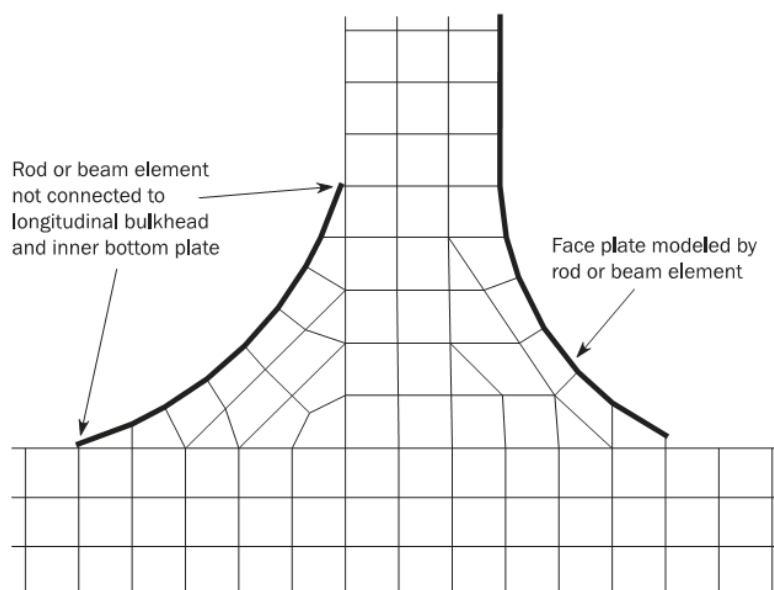
Figure 9 Typical finite element mesh on transverse web frame main bracket
