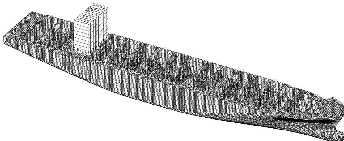
Figure 4 Global model with stiffener spacing mesh in cargo region/midship/ramp opening or within entire model extent
