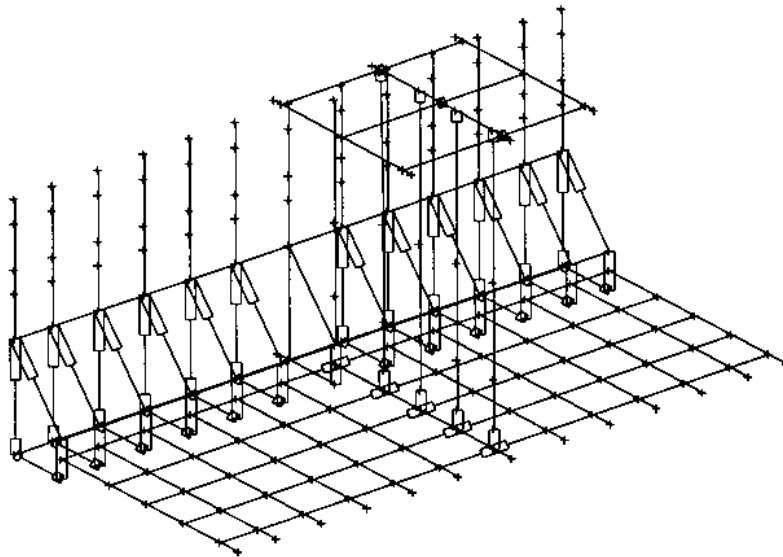
Figure 11 3D beam element model covering double bottom structure, hopper region represented by shear panels, bulkhead and deck between hatch structure. The main frames are lumped.
