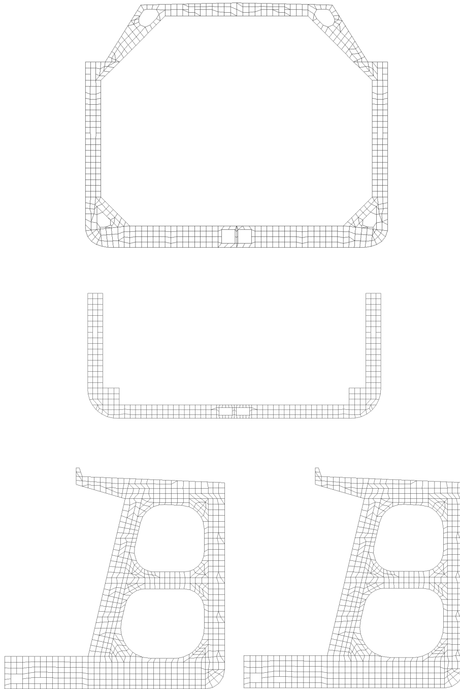
Figure 6 Typical finite element mesh on web frame of different ship types
