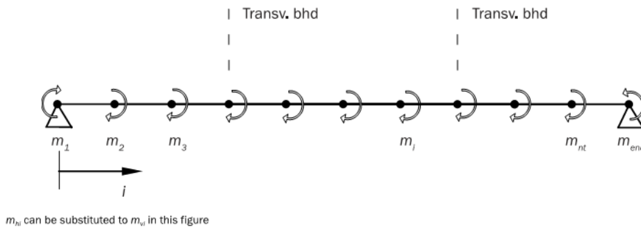
Figure 19 Adjustments of bending moments outside midship cargo hold region.
