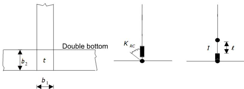
Figure 3 Non-bracketed corner model
