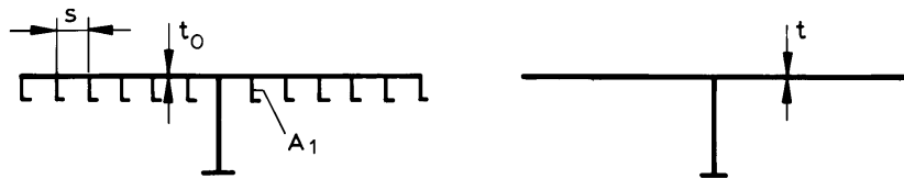
Figure 5 Equivalent flange thickness of single skin girder with stiffeners parallel to the web
