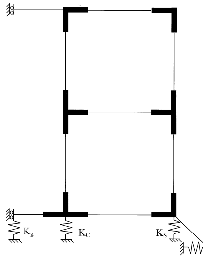
Figure 13 Transverse frame model of a ship with two longitudinal bulkhead
