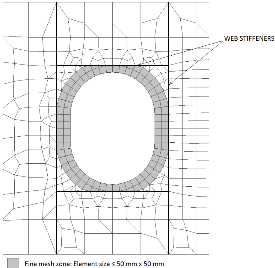
Figure 2 Fine mesh zone around an opening
