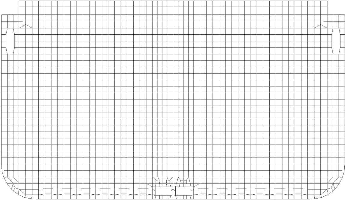
Figure 7 Typical finite element mesh on transverse bulkhead
