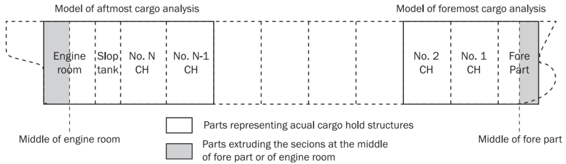
Figure 1 Hull form simplification for foremost and aftmost cargo hold model
