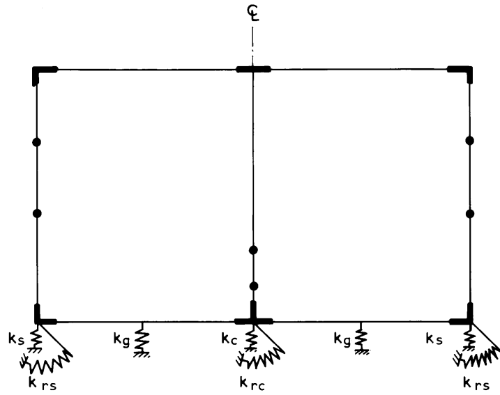
Figure 14 Transverse frame model of a ship with one longitudinal bulkhead
