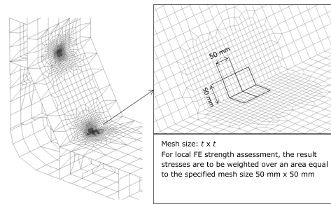
Figure 5 FE model of lower and upper hopper knuckles with mesh size t \times t used for local fine mesh strength analysis
