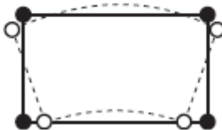
Figure 2 Improved bending of web modelled with one element over height
