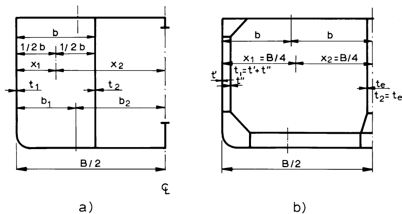
Figure 4 Hull girder sections
