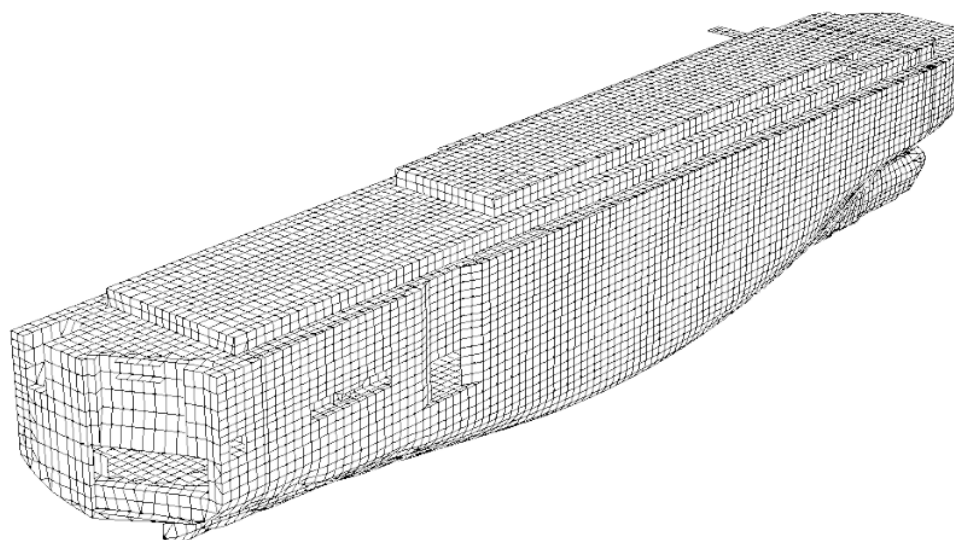
Figure 3 Typical global finite element model of a car carrier
