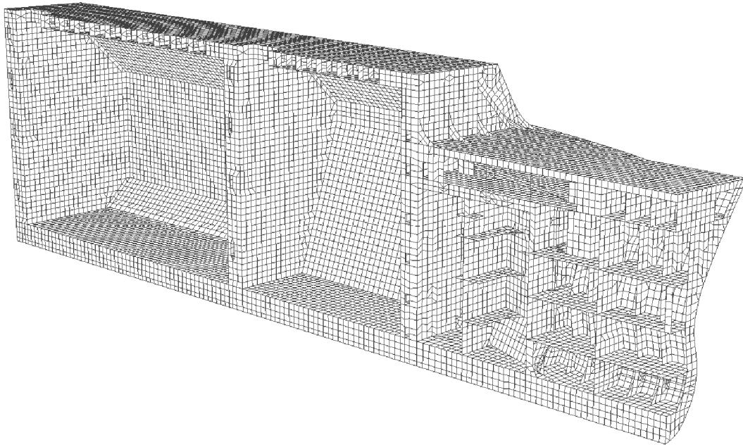
Figure 5 Example of FE model for the foremost cargo hold structure of a LNG carrier (membrane tank design) (shows only port side of the full breadth model)
