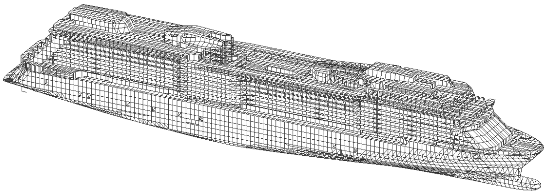
Figure 2 Typical global finite element model of a cruise vessel
