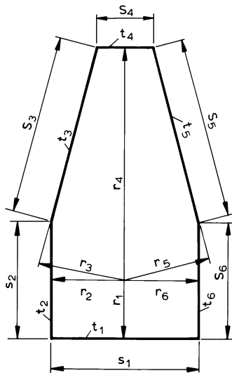
Figure 9 Definition of thickness and breadths for stool tank structure
