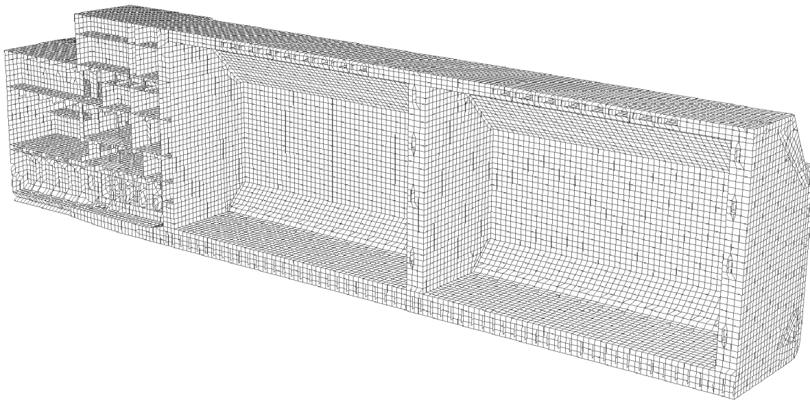
Figure 4 Example of FE model for the aftermost cargo hold structure of a LNG carrier (membrane tank design) (shows only port side of the full breadth model)
