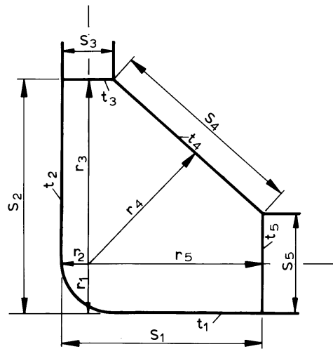
Figure 10 Definition of thickness and breadths for hopper tank structure
