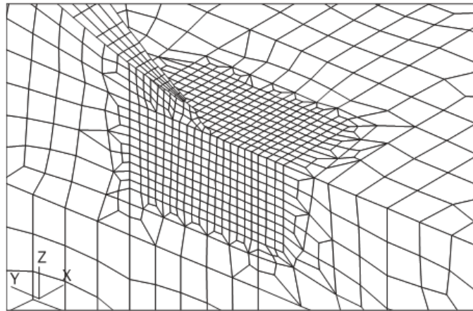
Figure 3 Fine mesh zone around bracket toes
