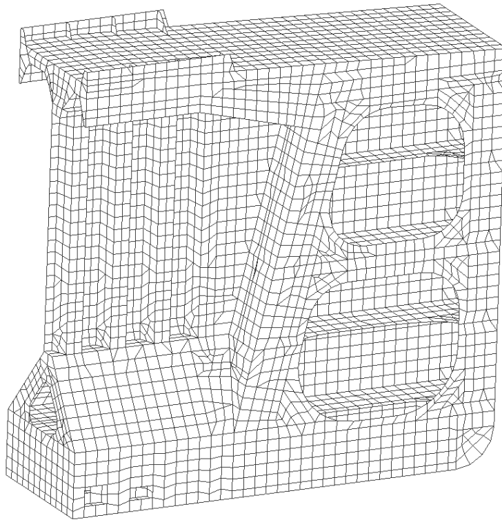
Figure 12 Example of FE mesh on transverse bulkhead structure for an ore carrier
