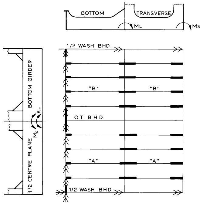
Figure 16 Bottom grillage model of a ship with two longitudinal bulkheads
