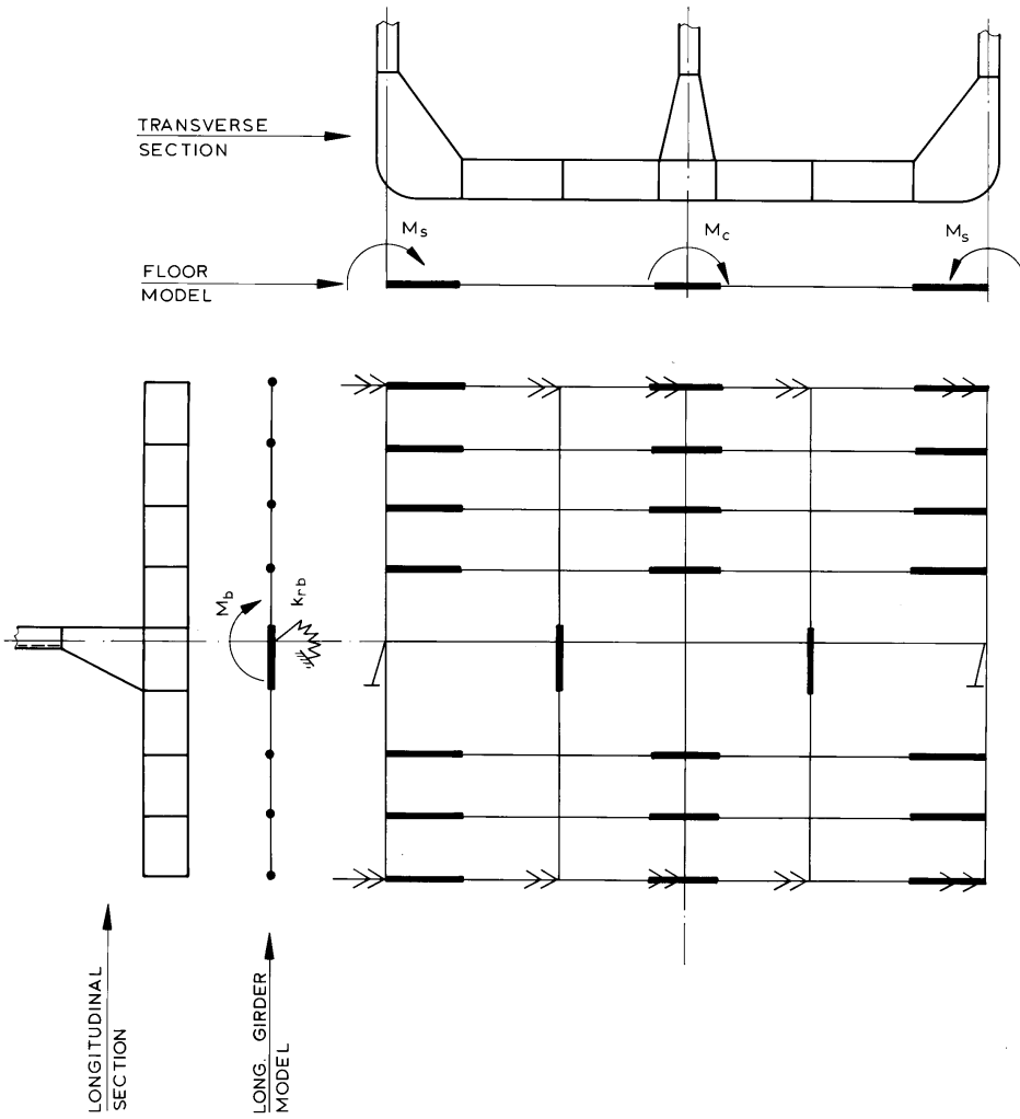
Figure 15 Bottom grillage model of a ship with one longitudinal bulkhead
