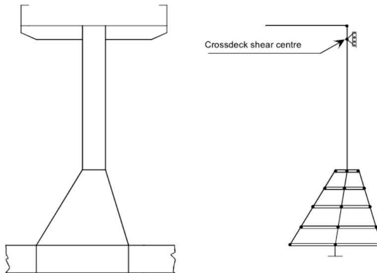
Figure 17 Two-dimensional beam model of vertical corrugated bulkhead (see also Figure A-19)
