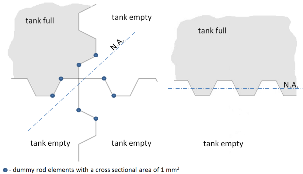
Figure 10 Example of dummy rod elements at the corrugation.
