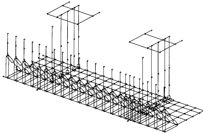
Figure 12 3D beam element model covering double bottom structure, hopper region, bulkhead and deck between holds. The main frames are lumped.
