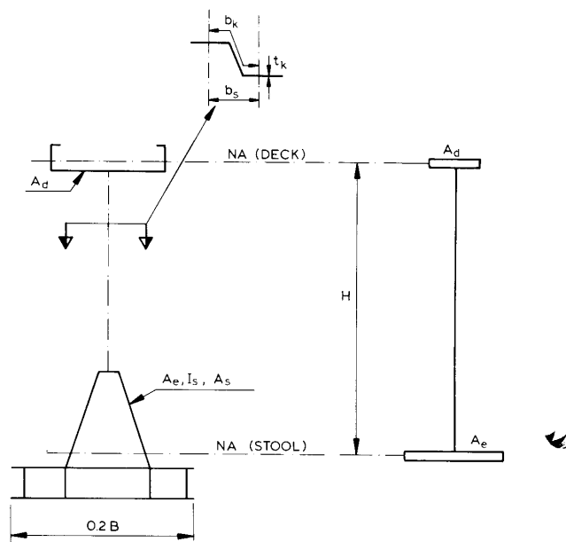
Figure 6 Cross-sectional data for bulkhead
