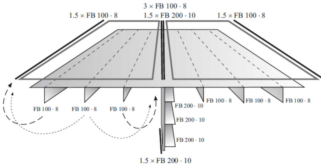
Figure 5 Example of plate and stiffener assemblies
