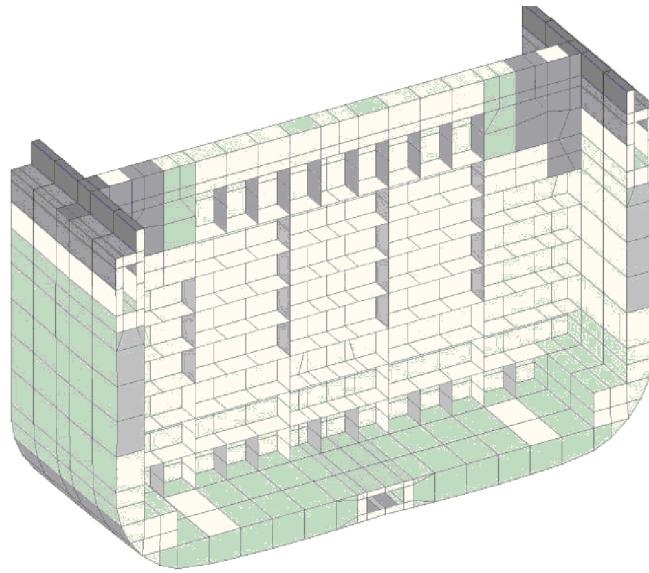
Figure 8 Typical midship mesh used for global finite element analysis of a container ship
