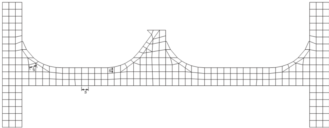
Figure 7 Typical finite element mesh on transverse bulkhead
