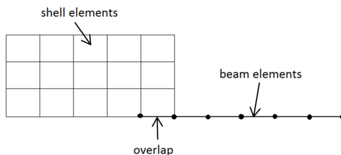
Figure 1 Overlap beam element in the transition between shell elements and beam elements representing stiffeners
