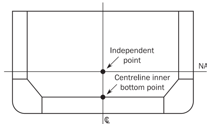
Figure 17 Boundary conditions applied at the model end sections
