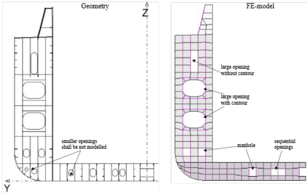
Figure 15 Modelling of openings in a transverse frame
