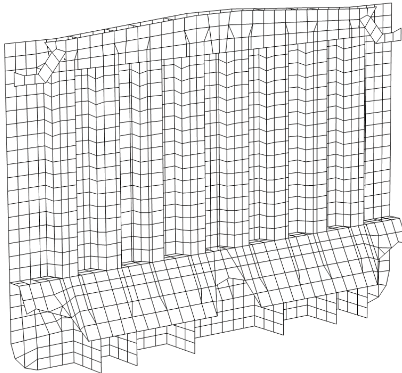
Figure 11 Example of FE mesh on transverse corrugated bulkhead structure for a product tanker
