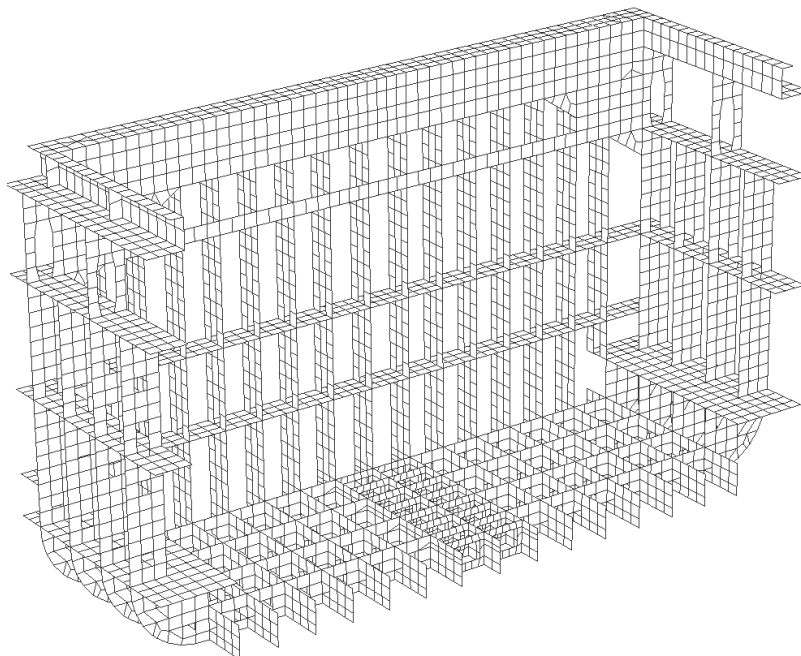
Figure 14 Example of FE mesh arrangement of cargo hold structure for a container ship
