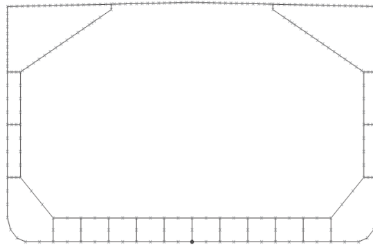
Figure 18 Example of end constraint beams for a bulk carrier
