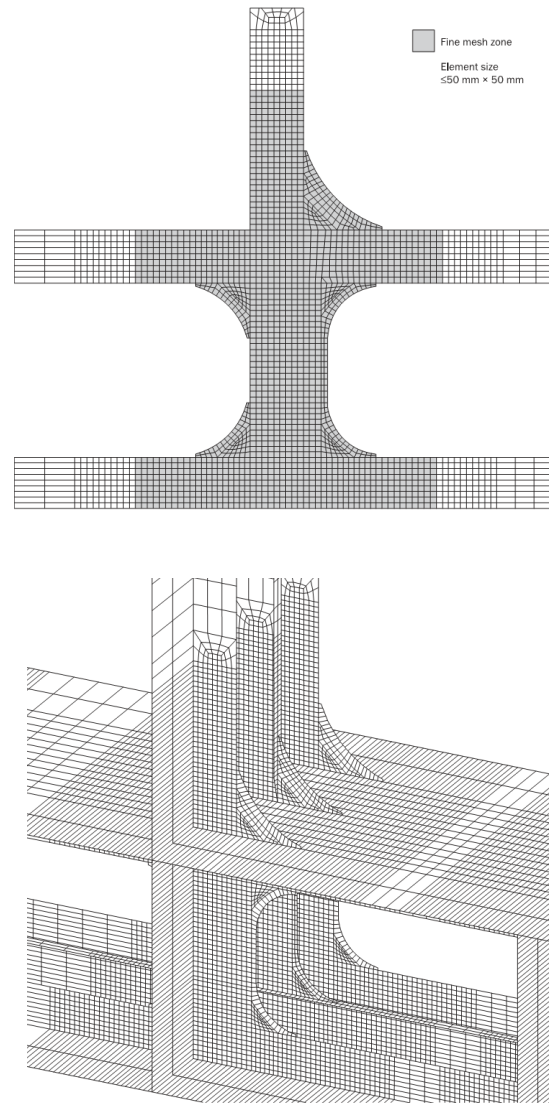
Figure 4 Example of local model for fine mesh analysis of end connections and web stiffeners of deck and double bottom longitudinals
